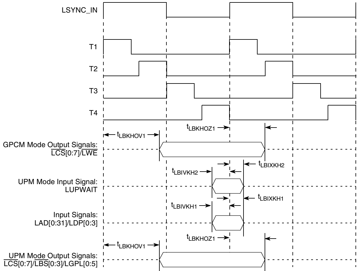
Figure 21. Local Bus Signals, GPCM/UPM Signals for LCCR[CLKDIV] = 4 or 8 (DLL Enabled)
